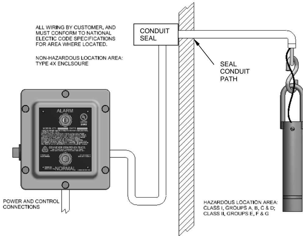
Figure 8: Typical CT-105 and CT-201G Probe Application with Different Environments
