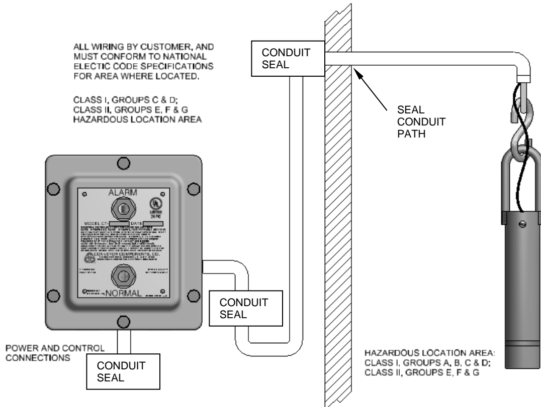
Figure 10: Typical CT-107 and CT-201G Probe Application with Different Environments
