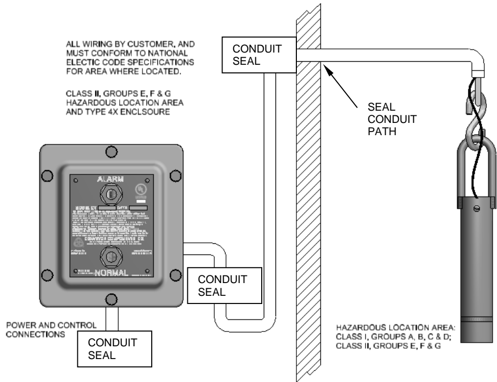
Figure 9: Typical CT-106 with CT-201G Probe Application with Different Environments
