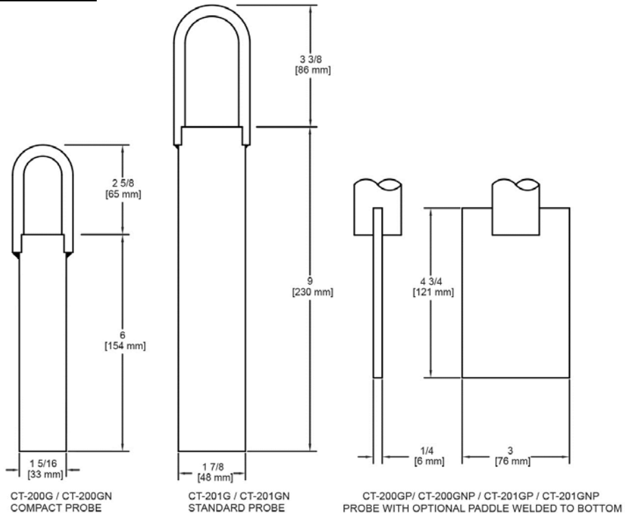
Figure 4: Probe Dimensions
