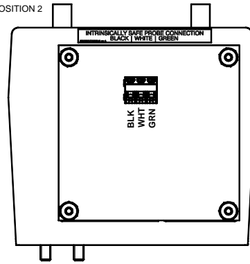
Figure 3: Control Board Probe Wiring Terminals
