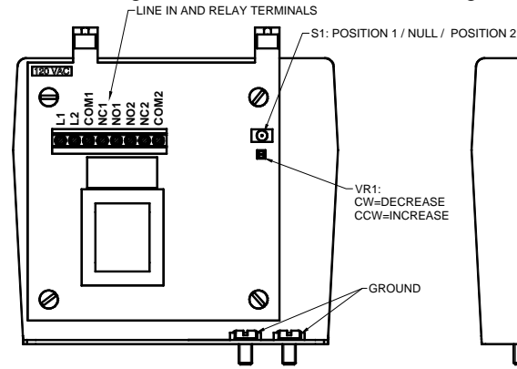
Figure 2: Control Board Wiring Terminals
